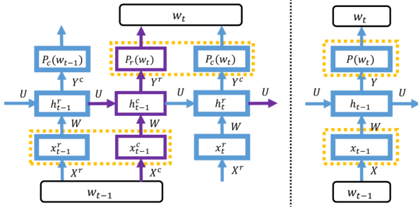
Fig. 1. LightRNN (left) vs. Conventional RNN (right). [3]
